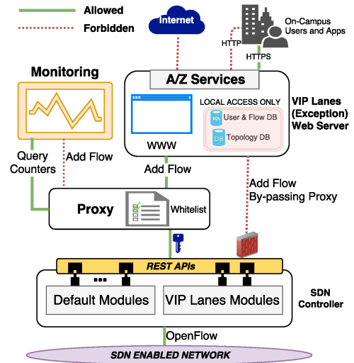
Fig. 2. Components of the VIP Lanes exception service, and allowed/forbidden communication among components.
