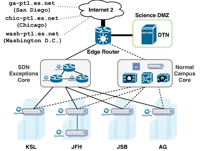
Fig. 3. SDN-enabled campus topology used to deploy exceptions
