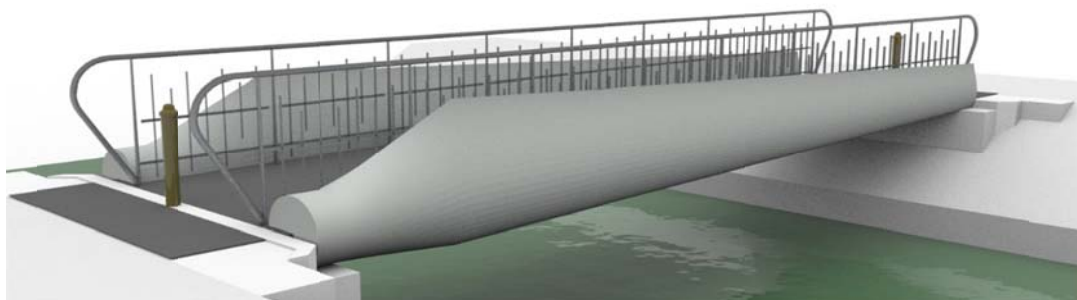
Figure 1: A conceptual design of pedestrian bridge using A29 windblades as main girders.
