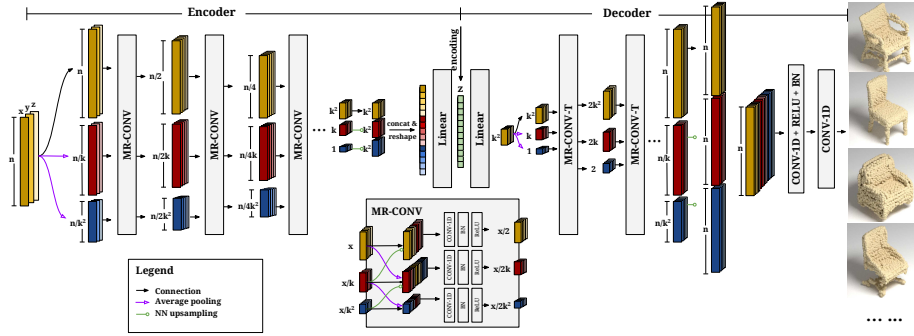
Fig. 2: Our multiscale tree network (MRTNet) for processing 3D point clouds. We represent a 3D shape as a 1D list of spatially sorted point cloud. The network represents each layer at three scales (indicated by yellow, red, and blue), the scale ratio is k between each two. The last two convolution layers have kernel size 1 and stride 1. MR-CONV refers to multi-resolution convolution (zoom-in to the inset for details); and MR-CONV-T refers to MR-CONV with transposed convolution. Our network is flexible and can be used for several shape processing tasks.
