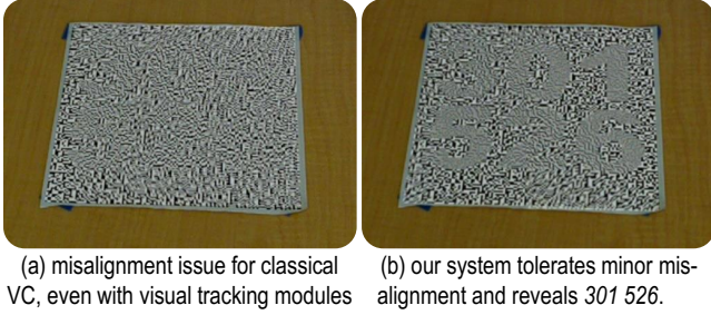
Figure 3: (a) A real case of misalignment challenge for classical visual cryptography using augmented reality headsets. As long as a single line is not aligned, the secure message will not be revealed. (b) In contrast, our system tolerates such minor misalignment by diffusing the second share using the normalized probabilities. Both images are captured with Magic Leap One’s Capture Service. Visual tracking is enabled for aligning the two shares in the head-mounted display but we still observe a slight jitter that throws off the conventional visual cryptography.
