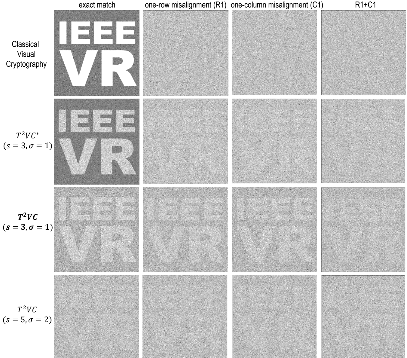
Figure 4: Results among the classical visual cryptography approach and T^2VC approaches with different parameters ( s indicates the size of the Gaussian kernel, \sigma indicates the standard deviation of the Gaussian kernel). From the results, we observe that both T^2VC and T^2VC^* outperform the visual cryptography algorithm in R1 or C1 cases. T^2VC provides better contrast than T^2VC^* when both R1 and C1 misalignment occur.
