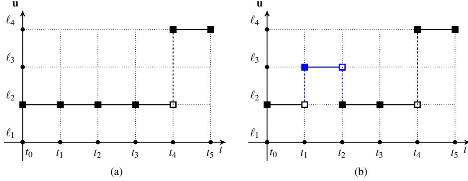
Fig. 6 (a) Example of using a finite-grid to approximate an input signal. The input signal u(t) is obtained by constant interpolation over the sequence (\ell_2, \ell_2, \ell_2, \ell_2, \ell_4, \ell_4) over the time-domain (t_0, t_1, t_2, t_3, t_4, t_5) . (b) Example of a grid-neighbor of the input signal shown in (a).
