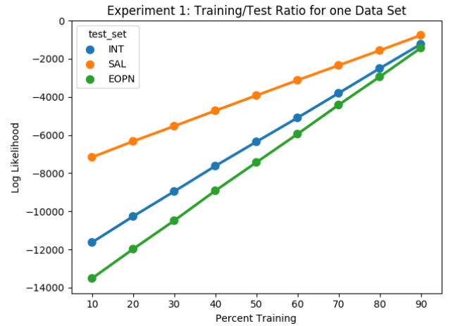
Figure 1: Experiment 1: Log-likelihood when varying ratio of training to test data.
