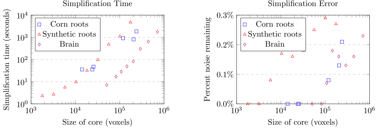
Figure 4: (a) Experimental runtime and (b) error rates on three datasets.
