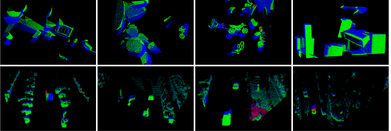
Figure 5: Qualitative results on FlyingThings3D (top) and KITTI (bottom). Blue points are PC_1 , green points are correctly predicted (measured by Acc3D Relax) flowed points PC_1 + \widehat{sf} , and red points are ground-truth flowed points PC_1 + sf which are not correctly predicted. Note that the objects in the two datasets have very different motion patterns, which shows our method’s generalization ability. The third figure of the second row shows that some failures are on the ground, which suggests the performance on KITTI may be further improved by better ground removal algorithms.
