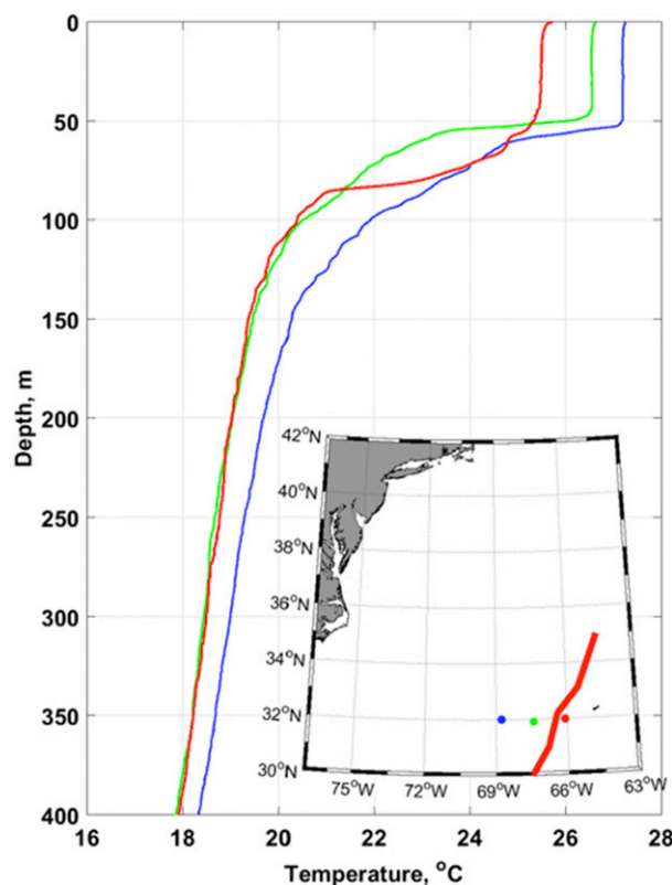
FIG. 8. Three XBT profiles taken from the Oleander as it passed behind Hurricane Joaquin. The blue profile is \sim 200 km west of the hurricane path, the green one is at the western flank, and the red one is just east of the hurricane center, where the winds are very strong. The red line shows the path of the center of the hurricane.
