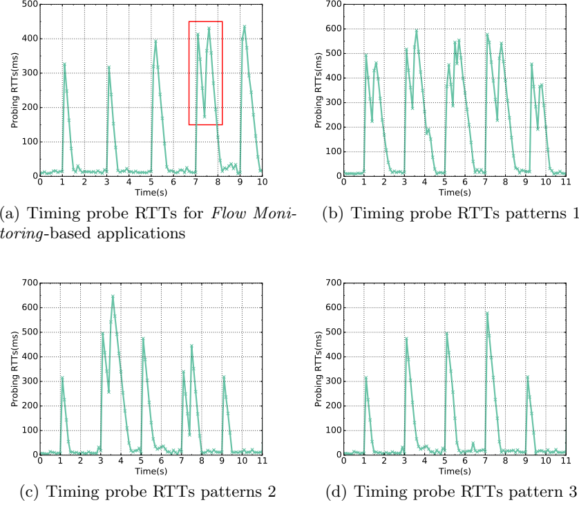
Fig. 6: Timing-based Patterns for Counter Manipulation Attack
