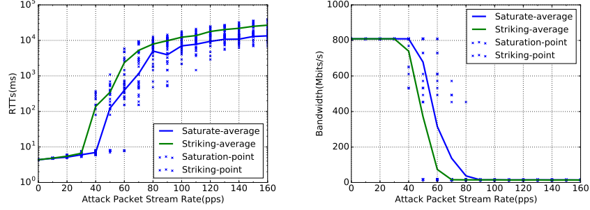
(a) RTTs for normal users under the saturation attack and the striking attack (b) Bandwidth for normal users under the saturation attack and the striking attack Fig. 5: RTTs and Bandwidth for normal users under the saturation attack and the striking attack
