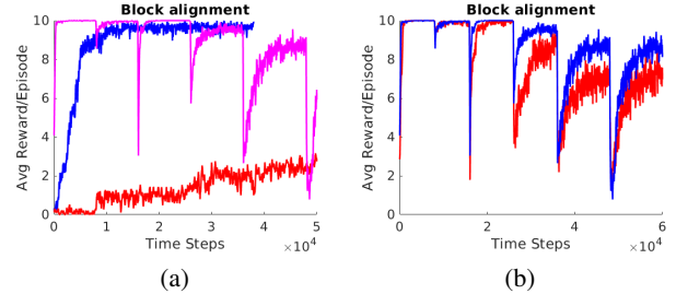
Figure 5: (a) Ablation of curriculum learning. Blue, red: learning curves for curriculum stages 4 and 5, respectively, without running stages 1–3 first. Magenta: learning curve with curriculum. (b) Ablation of hierarchical value function. Blue: WITHOUT Q-function hierarchy; Red: WITH Q-function hierarchy.
