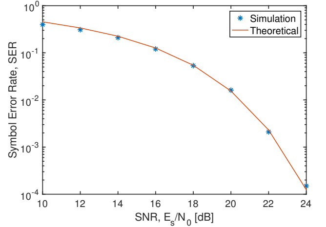
Fig. 9: SER as a function of SNR for closer receiver.
