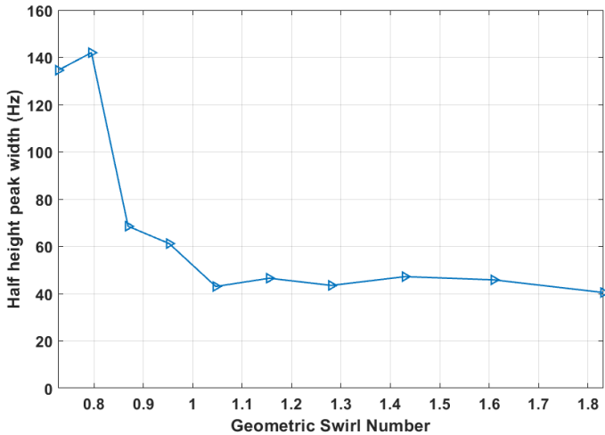
FIGURE 8. Peak width at half the peak height of the first SPOD mode frequency domain spectra.
