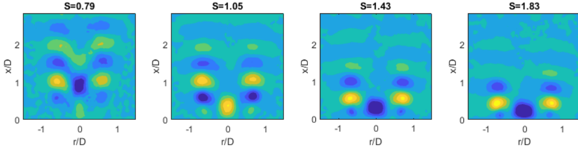
FIGURE 6. SPOD mode shapes of the first mode for select swirl numbers at their respective PVC frequencies.
