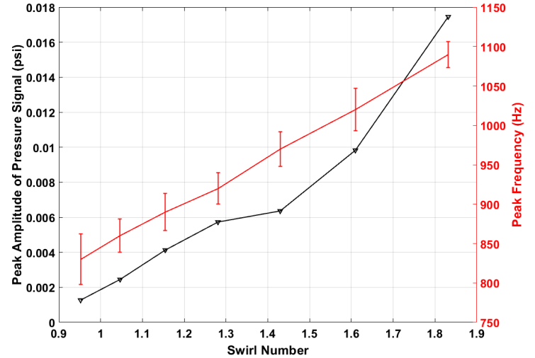
FIGURE 3. Variation in PVC frequency and amplitude (with error bars representing the peak width) obtained from pressure transducer data.
