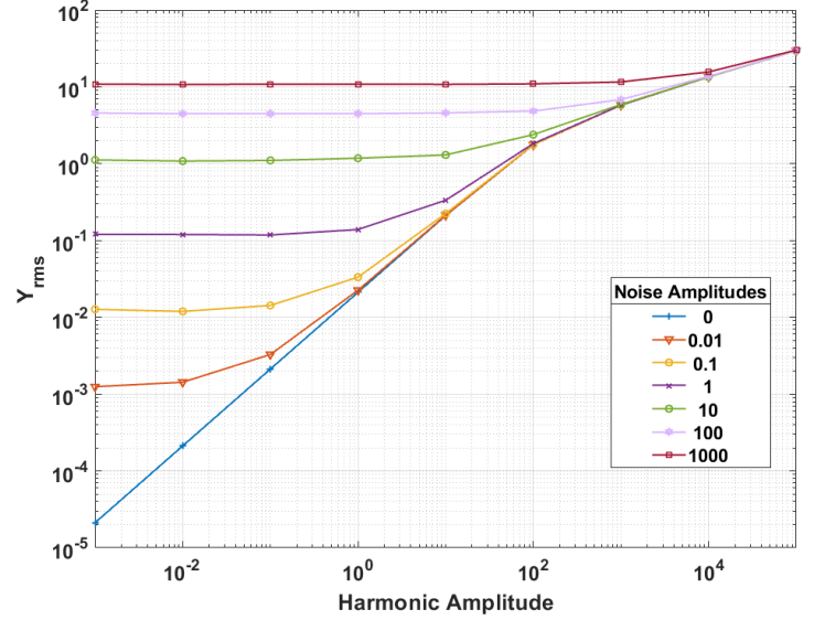
FIGURE 9. RMS of the solution of a van der Pol forced by noise and a harmonic forcing function.
