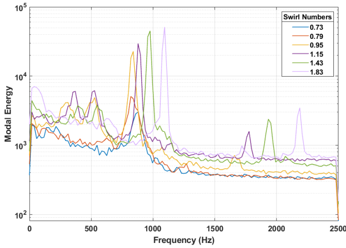
FIGURE 7. Modal energy spectra of the first SPOD mode.
