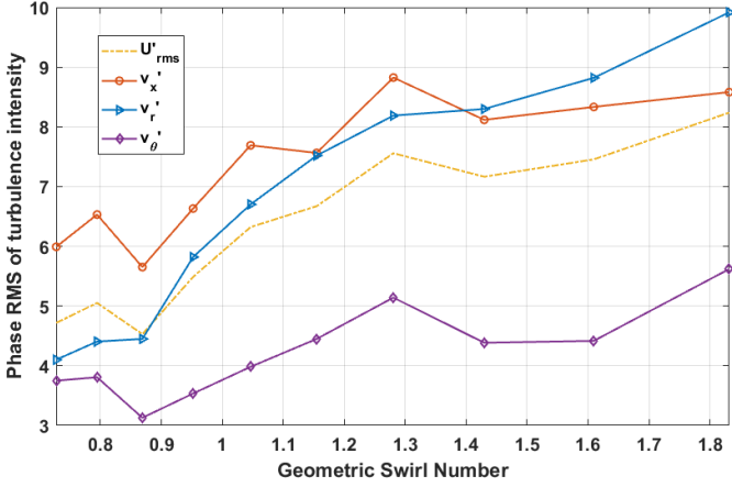
FIGURE 5. Variation in turbulence intensity at the mean vortex location with swirl number.
