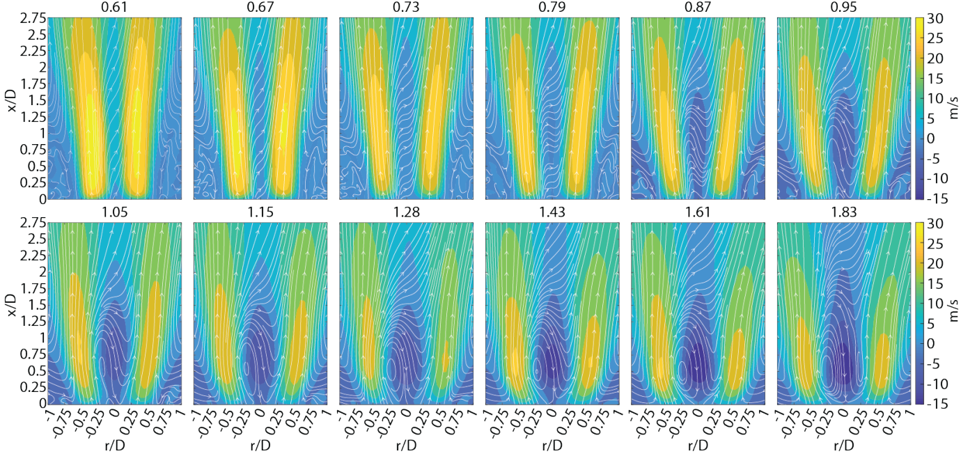
FIGURE 2. Time-averaged axial velocity contours and streamlines at a range of swirl numbers.
