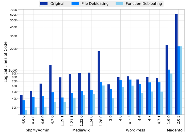
Figure 3: Logical Lines of Code before and after debloating
