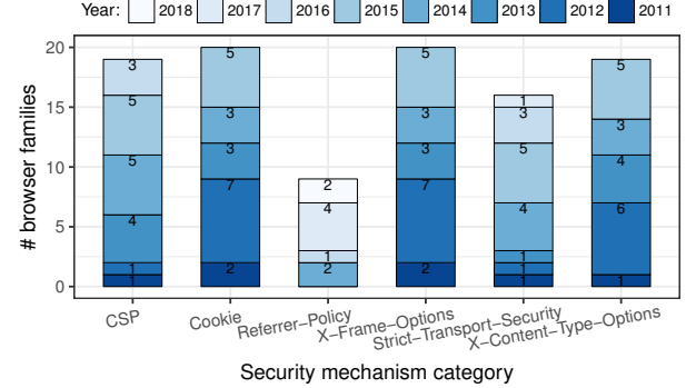
Fig. 7: Adoption rate of security mechanisms over the years.
