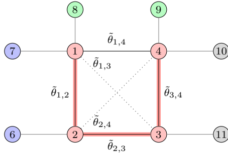
Fig. 2. For the cluster with nodes \mathcal{C} = \{1, 2, 3, 4\} in Fig. 1, this figure shows a spanning tree \mathcal{T} = (\mathcal{C}, \mathcal{E}_{\mathcal{T}}) , where \mathcal{E}_{\mathcal{C}} = \{(1, 2), (2, 3), (3, 4), (1, 4)\} . The system (8) associated with the cluster \mathcal{C} is in Example 1.
