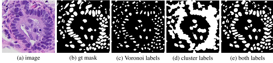
Figure 3: Results using different pixel-level labels: (a) image, (b) ground-truth mask, (c)-(e) are results using Voronoi labels, cluster labels and both labels, respectively.
