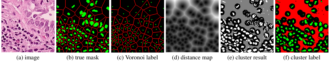
Figure 2: Label generation. (a) original image, (b) ground-truth nuclei masks (in green) and Voronoi edges (in red), (c) Voronoi label, (d) distance map, (e) clustering result, (f) cluster label (green: nuclei, red: background, black: ignored).
