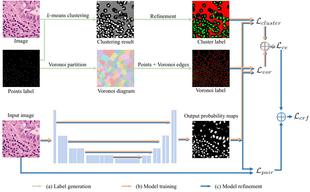
Figure 1: Overview of the proposed approach. (a) Label generation. The Voronoi label and cluster label are generated using the points label and original image. The green, red and black colors indicate nuclei, background and ignored pixels, respectively. (b) Model training using the cross entropy loss. (c) Model refinement using the CRF loss.
