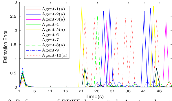
Fig. 3: Performance of RDKF during attack. Agents under attack are marked with (a). Estimation error is bounded and small.
