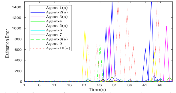
Fig. 5: Performance of non RDKF during attack. Agents under attack are marked with (a). Estimation error is large.
