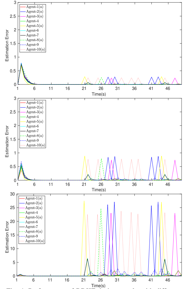
Fig. 4: Performance of RDKF during attack, with different parameter values. The three figures correspond to small value of \lambda , large value of \Sigma_v and large value of \Sigma_w respectively.
