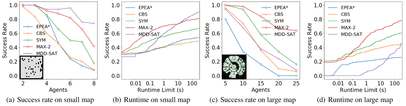
Figure 3: Experimental results on 2D grids.
