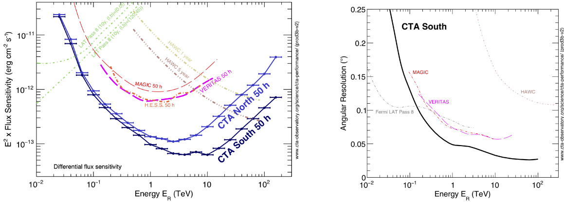
Figure 3: Comparisons of the CTA performance with selected existing \gamma -ray instruments. Left: differential energy flux sensitivities for CTA (south and north) for five standard deviation detections in five independent logarithmic bins per decade in energy. For the CTA sensitivities, additional criteria are applied to require at least ten detected \gamma -rays per energy bin and a signal/background ratio of at least 1/20. The Fermi -LAT and HAWC curves are scaled by a factor of 1.2 to account for different energy binning. The curves shown give only an indicative comparison between the different instruments, as the method of calculation and the criteria applied are different. In particular, the definition of the differential sensitivity for HAWC differs due to the lack of energy reconstruction for individual photons in the HAWC analysis from which this curve is taken [21]. Right: angular resolution expressed as the 68% containment radius of reconstructed \gamma -rays (the resolution for CTA-North is similar). These plots represent the understanding of the performance of CTA at the time of completion of this document; for the latest CTA performance plots, see https://www.cta-observatory.org/science/cta-performance .
