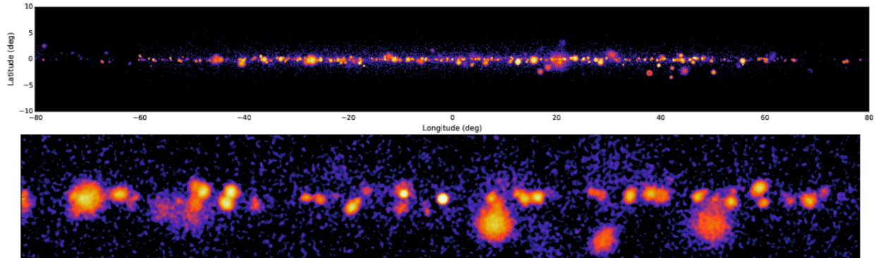
Figure 2: Top: simulated CTA image of the Galactic plane for the inner region, -80^\circ < l < 80^\circ , adopting the proposed Galactic Plane Survey Key Science Project observation strategy and a source model incorporating both supernova remnant and pulsar wind nebula populations, as well as diffuse emission. Bottom: a zoom of an example 20^\circ region in Galactic longitude. [6]
