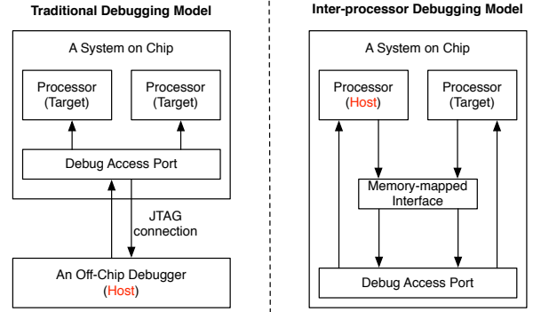
Figure 1: Debug Models in ARM Architecture.
