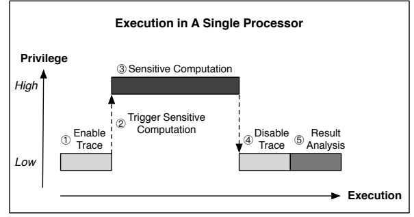
Figure 4: Violating the Isolation via Non-Invasive Debugging.
