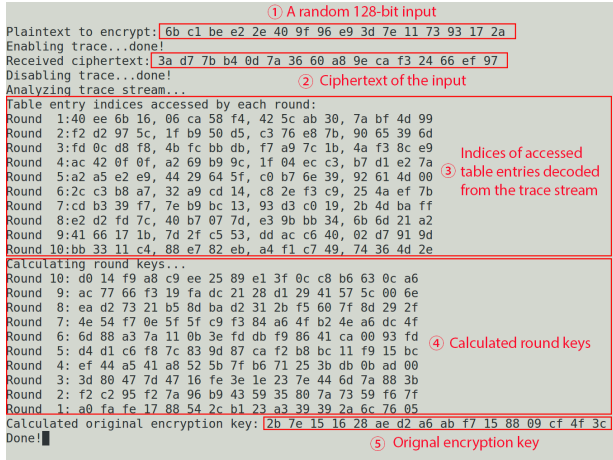
Figure 6: Retrieving the AES Encryption Key.
