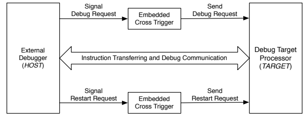
Figure 3: Invasive Debugging Model.
