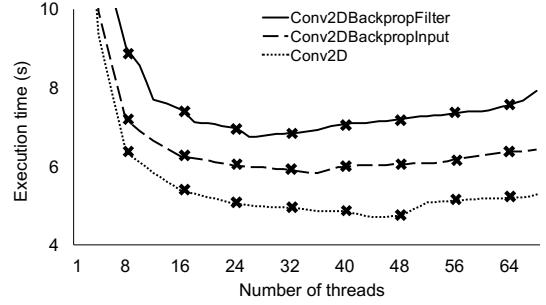
Fig. 1: Performance variance of three operations with different intra-op parallelisms. The reported execution time is the total execution time of one thousand runs.
