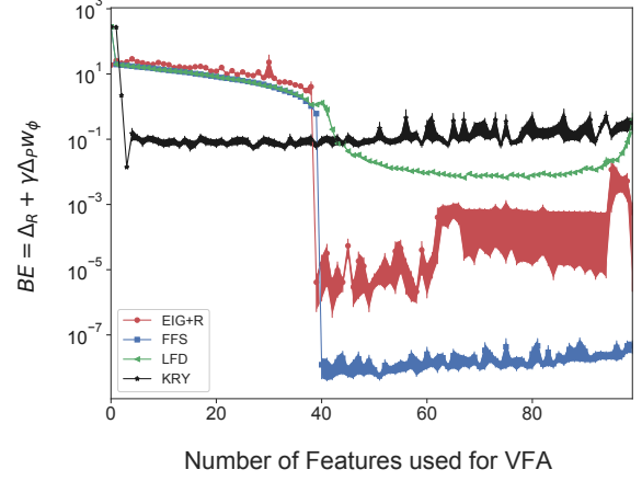
Figure 2: Bellman error for the approximate solution. The transition matrix is 100 \times 100 and has a low rank with \text{rank}(P) = 40 . The Input matrix is A = \text{random binary matrix} .
