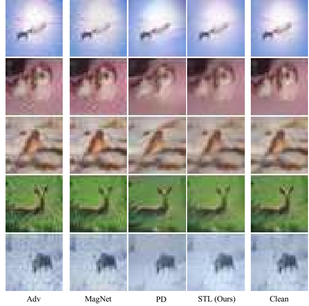
Figure 4: Qualitative comparison on CIFAR-10 [23] with MagNet [32] and PixelDefend (PD) [46]. The first column is adversarial images generated by FGSM [18] with L_2 -dissimilarity = 0.08. The last column is corresponding clean images. We can observe that MagNet cannot fully remove adversarial perturbation, while PixelDefend over-smooths images, causing large information loss and sometimes introducing colorful artifacts.
