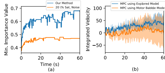
Fig. 5: (a) Comparison of the minimum importance measure of the data set for the half-cheetah example from a stable standing policy with added 20% saturation limit noise and our approach for active data acquisition. (b) Integrated forward velocity values from using the learned half-cheetah dynamics model in a model-predictive control setting with standard deviation illustrated for 5 trials. Our method is shown to collect data which provides a better dynamic model and a positive net forward velocity with reduced variance.
