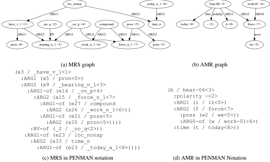
Figure 1: The graphs and PENMAN notations of MRS and AMR for the sentence “it<0> has<1> no<2> bearing<3> on<4> our<5> work<6> force<7> today<8>” (From wsj_0003-30).
