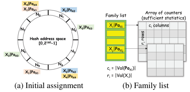
Figure 1: Assignment of families to cluster nodes
