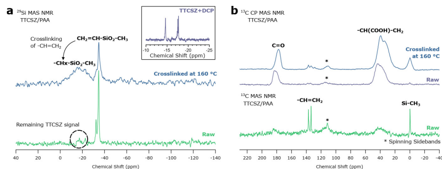
Figure 9. Solid-state NMR spectra of TTCSZ/PAA hybrid raw fibers and crosslinked fibers. ^{29}\text{Si} MAS NMR result indicates decreased mobility after crosslinking, and ^{13}\text{C} showed very low interaction between PAA (rigid environment) and TTCSZ at crosslinking stage. Number of scans (NS): ^{29}\text{Si} MAS Crosslinked at 160^\circ\text{C} (NS = 474), Raw (NS = 140); ^{13}\text{C} CP MAS Crosslinked at 160^\circ\text{C} (NS = 1056), Raw (NS = 432); ^{13}\text{C} MAS Raw (NS = 56).
