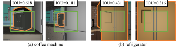
Figure 3: IOU between the target’s mask and the centered rectangle mask. Higher IOU is achieved when the target has larger portion in the center of the view.
