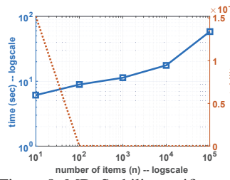
Figure 8: MD: Stability verification, Impact of dataset size
