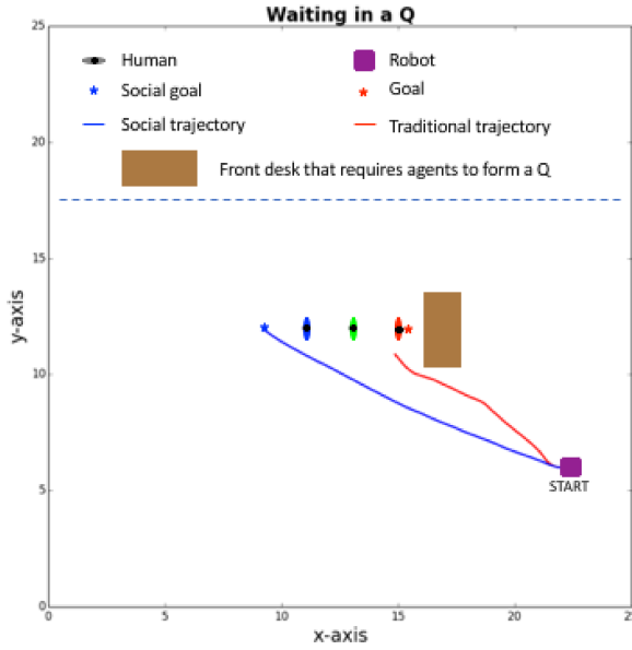
Figure 4: Showing PaCcET local planner (blue trajectory) in comparison with traditional local planner (red trajectory) in a “Waiting in a queue scenario”. Our approach steered the robot to join the line, whereas the traditional planner steered the robot to the front of the desk.
