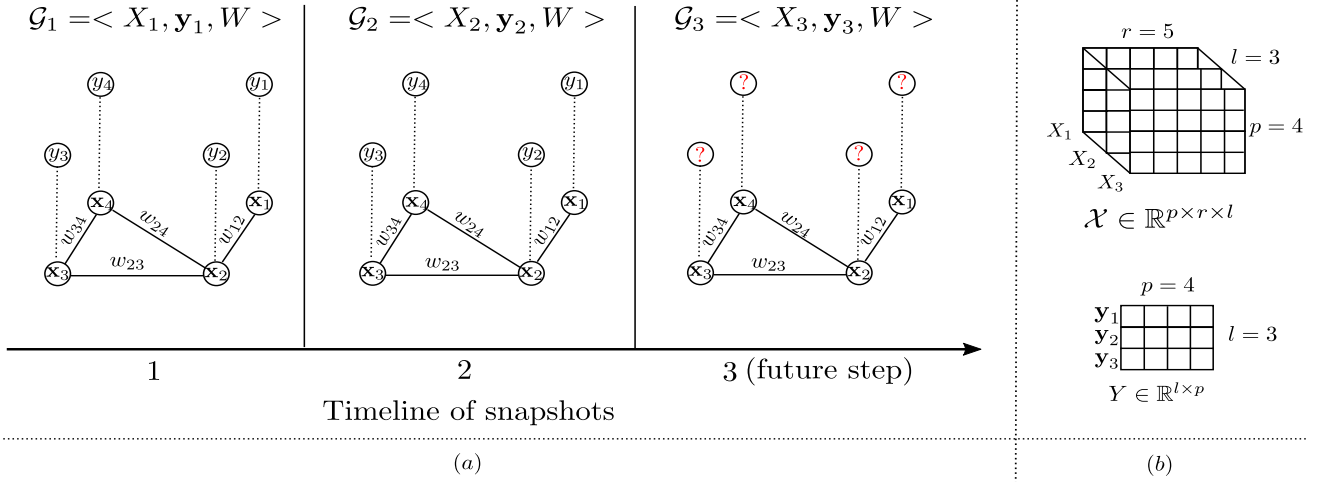
Figure 1: Illustration of temporal graph regression. (a) Temporal graph example with l = 3 snapshots, p = 4 nodes and r = 5 features in each node. \mathbf{x}_i is the vector of features of node i . \mathbf{y}_i is the target of node i . (b) Joint view of feature space and target space in \mathcal{G} .
