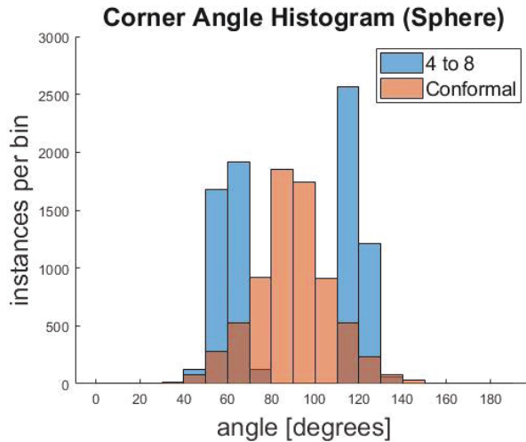
Fig. 2. Corner angle histogram for conformal remeshing and 4 to 8 subdivision for a sphere
