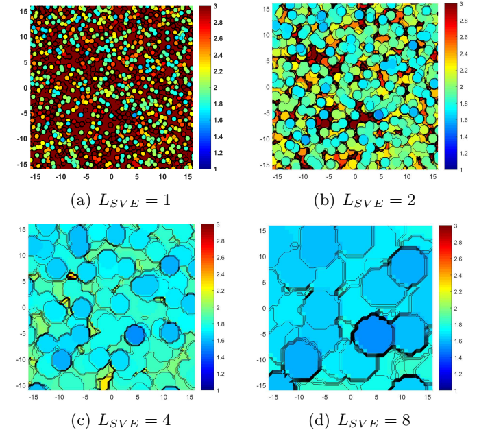
Figure 8: Random fracture strength fields for four SVE sizes at the same loading angle.
