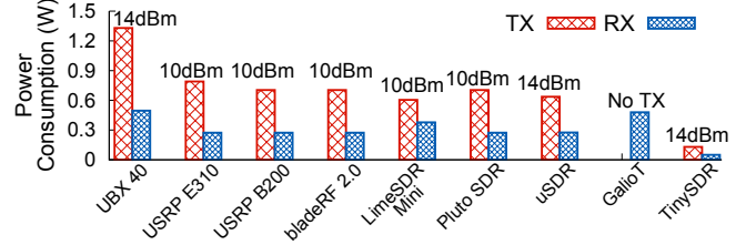
Figure 2: Radio Module Power Consumption for Each Platform. The TX output power of each radio module is shown on top of it.
