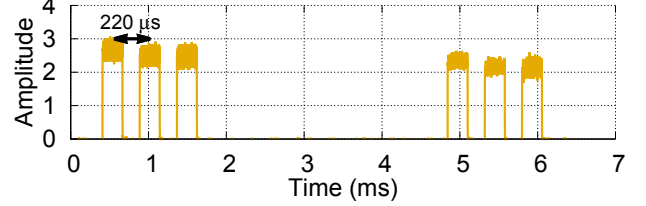
Figure 13: BLE Beacons Signal. We show BLE beacon transmissions on three advertising channels from tinySDR using an envelope detector.
