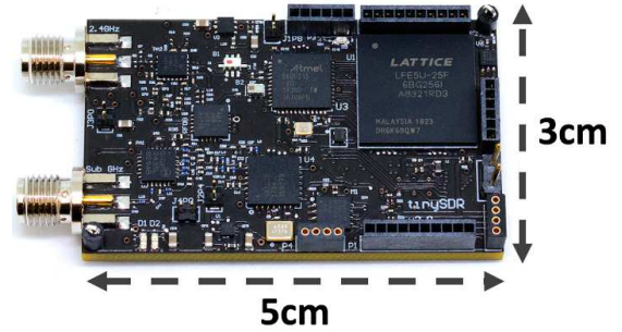
Figure 1: TinySDR Hardware Platform. It has two antenna ports for running IoT PHY and MAC protocols at 2.4 GHz and 900 MHz. This image is the actual size of the platform on printed paper.
