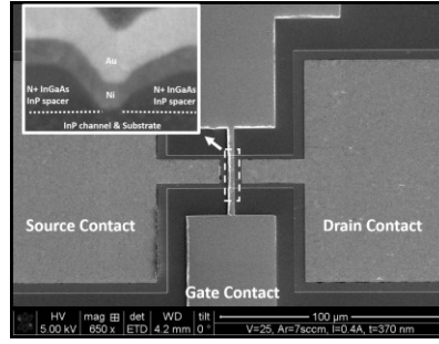
Fig. 2 Top view and cross-sectional SEM image of a device having ~40 nm L_g .
