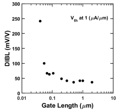
Fig. 8 DIBL vs. L_g .
