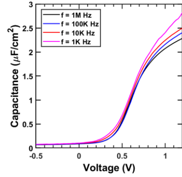
Fig. 3 CV characteristics of an InP MOSCAP with a ~4 nm ZrO_2/AlO_xN_y gate dielectric
