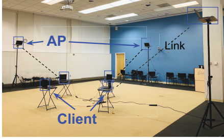
Fig. 3: Setup of 4 links in a 36ft×36ft classroom
