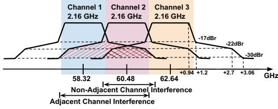
Fig. 4: Channelization can effectively reduce the interference between links but adjacent and non-adjacent channel interference cannot be neglected when clients are close to each other.
