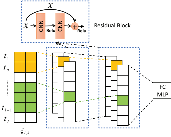
Figure 2: Our discriminator’s structure follows a one-dimensional CNN architecture in line with (Gulrajani et al. 2017). The input is l length sequence, where each element has k features. In the figure k = 2 , while in our paper, k = 1 , which is the inter-event time duration.
