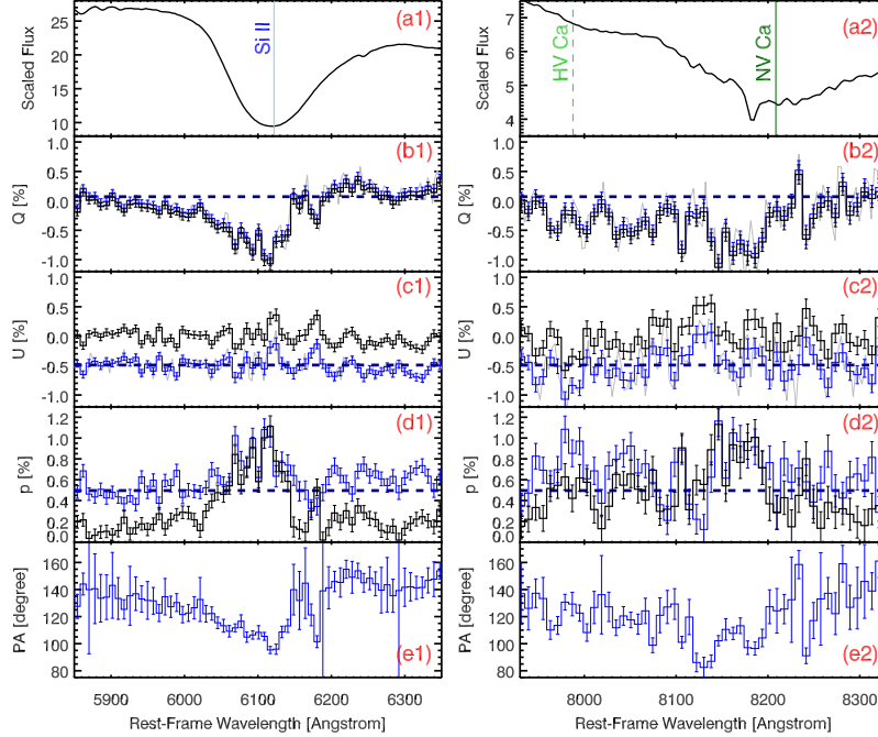
Figure 20. Same as Fig. 15, but on the spectropolarimetry of SN 2018gv across Si II \lambda 6355 (the left panels) and the Ca II NIR3 (the right panels) at day -0.5 (epoch 2). The data have been rebinned to 8\text{ \AA} . In the left panels, i.e. d1, the Si II polarization declines much faster from its peak around \sim 6200\text{ \AA} ( v \sim -11,000\text{ km s}^{-1} ) towards longer wavelengths compared to shorter wavelengths. Multiple peaks around \sim 6100\text{ \AA} may indicate the presence of various Si-rich components, which were not identified in the flux spectrum.
