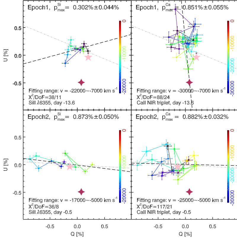
Figure 18. The polarization for the Si II \lambda 6355 (left panels) and the Ca II NIR3 (right panels) features on the Stokes Q-U plane at -13.6 day and -0.5 day. The data have been rebinned to 25 \text{ \AA} . In each panel, the points are color coded according to the velocity relative to the respective wavelengths measured in the rest frame for the two features. The data were corrected for the ISP (the location of which is indicated by the filled maroon star) and the continuum polarization is shown by the solid pink \star . The maximum polarization across the feature after ISP-correction is also presented. The dashed black line fits the displayed data points and the dotted gray line traces the dominant axis computed in the wavelength range 4300 \leq \lambda \leq 9100 \text{ \AA} .
