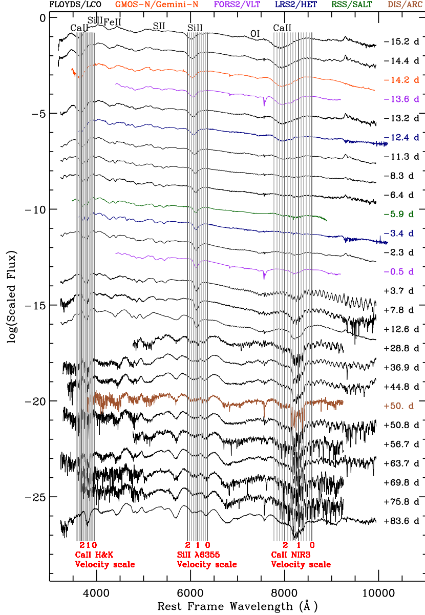
Figure 6. Spectral time series of SN2018gv (solid curves, phase is label on right). The wavelengths corresponding to 0 \text{ km s}^{-1} , -10,000 \text{ km s}^{-1} and -20,000 \text{ km s}^{-1} around the features indicated by the text are shown as thick gray lines, with 2000 \text{ km s}^{-1} intervals denoted by thin gray lines. For the purpose of presentation, all spectra were binned to 3 \text{ Å} .
