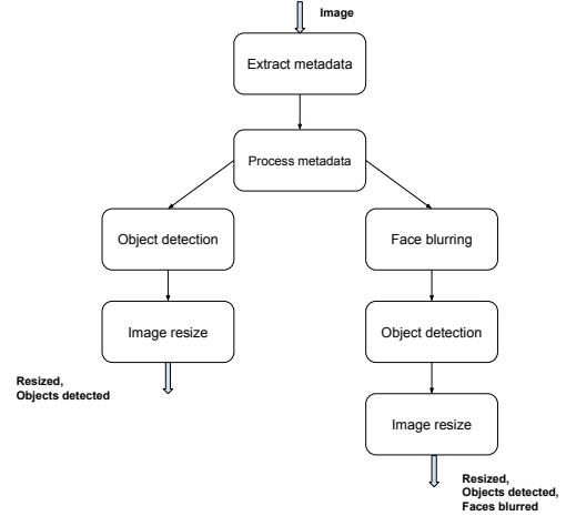
Figure 1: A motivating example showing an image processing pipeline
