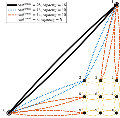
Figure 3: The basic traffic graph. AGVs are initialized at 0 and 1, traveling to the opposite vertex, i.e. vertex 1 or vertex 0, respectively. Edges (0, 1), and (1, 0) have the highest capacity and represent the shortest path. The goal of the multiagent traffic management team is to incentivize AGVs to take detours to alleviate congestion. Figure from [4].
