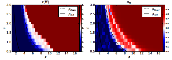
Figure 5. Left frame: Empirical fraction of instances such that V(\hat{W}) \geq \varepsilon_0 = 5 \cdot 10^{-3} , where \hat{W} is the AMP estimate. Here k = 2, d = 1000 , and for each (\delta, \beta) point on the grid we ran AMP on 400 random realizations. Right frame: Binder cumulant for the correlation between AMP estimates \hat{W}, \hat{H} and the true weights and topics W, H . Here k = 2, d = 1000 and estimates are obtained by averaging over 400 realizations.
