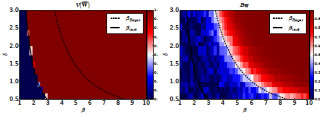
Figure 2. Gaussian model. Left frame: Empirical fraction of instances such that V(\widehat{W}) \geq \varepsilon_0 = 10^{-4} , where \widehat{W} is the naive mean field estimate. Here k = 2 , d = 1000 and, for each (\delta, \beta) point on a grid, we used 400 random realizations to estimate the probability of V(\widehat{W}) \geq \varepsilon_0 . Right frame: Binder cumulant for the correlation between the naive mean field estimate \widehat{W} , and the true weights W , H . Here k = 2 , d = 1000 and n = d\delta , and we averaged over 400 realizations. Solid lines: The instability curve \beta_{\text{inst}}(\delta) . Dashed lines: The Bayes phase transition \beta_{\text{Bayes}} .
