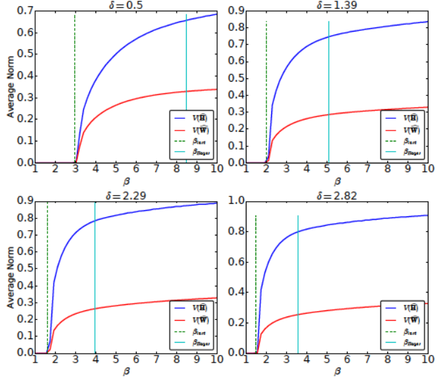
Figure 1. Normalized distances V(\hat{H}), V(\hat{W}) of the naive mean field estimates from the uninformative fixed point. Here k = 2 , d = 1000 and n = d\delta : each data point corresponds to an average over 400 random realizations.
