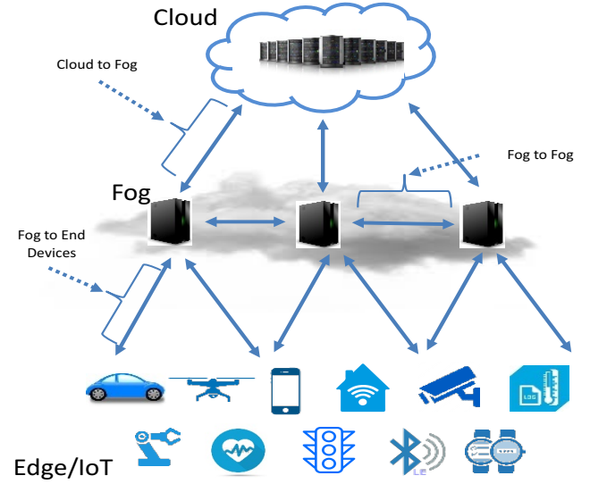
Fig. 3: Attack Surfaces
