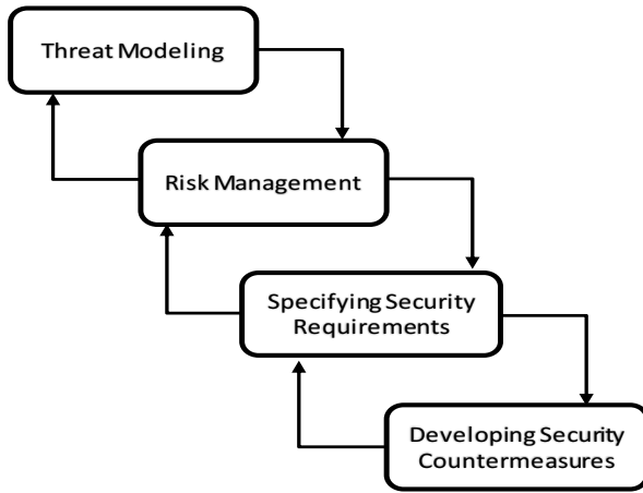
Fig. 1: Threat Modeling
