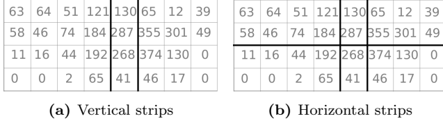
Figure 8: STR Spatial partitioning for the histogram.
