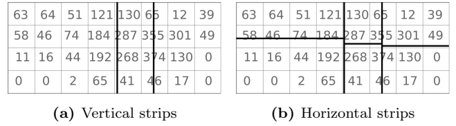
Figure 9: Spatial partitioning for the histogram partial cells.
