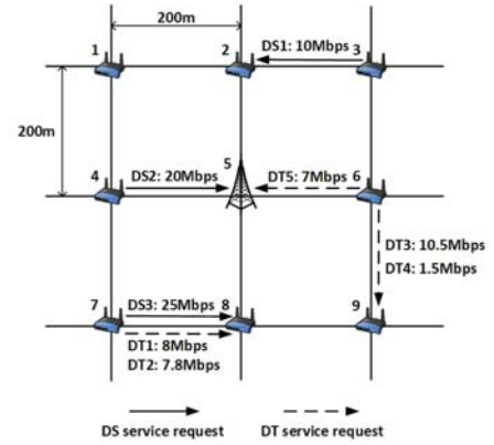
Fig. 3. A grid network with 9 nodes, 3 DS requests and 5 DT requests.
