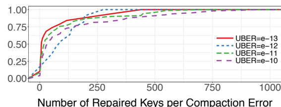
Figure 11: CDF of patch sizes generated during the ZippyDB-DIRECT recovery process. The patch size is small, which means low error amplification.
