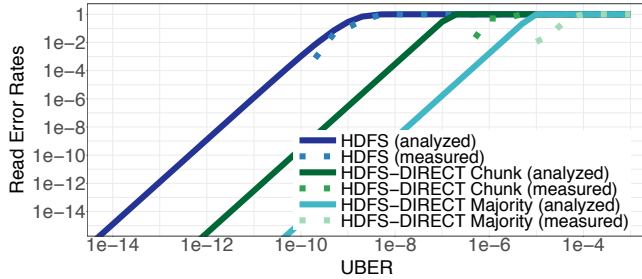
Figure 7: Read error rate for HDFS with varying UBER. HDFS-DIRECT Chunk is based on chunk-by-chunk recovery, while HDFS-DIRECT Majority is computed on bit-by-bit majority. The analyzed data is computed using the formulas in §3.
