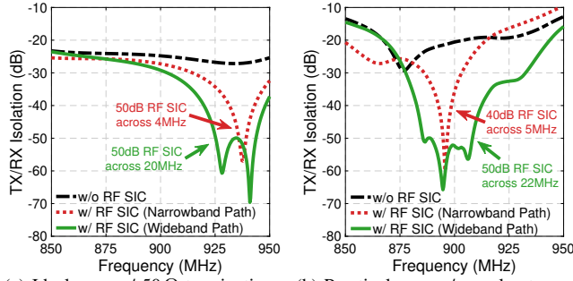
(a) Ideal case w/ 50\Omega termination. (b) Practical case w/ a real antenna. Fig. 3: Measured TX/RX isolation of the Gen-2 RF canceller without turning on the canceller, and with the narrowband (Gen-1)/wideband (FDE) path on, when the circulator antenna port is: (a) terminated by 50\Omega , and (b) connected to an antenna.
