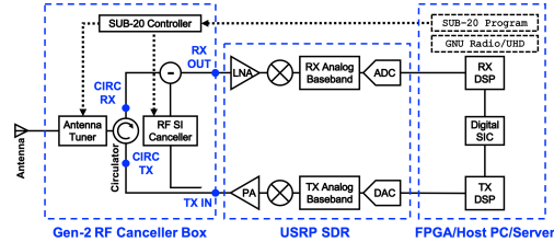
Fig. 1: Block diagram of the implemented Gen-2 wideband full-duplex (FD) radio consisting of a Gen-2 RF canceller box, a USRP software-defined radio (SDR), and a compute node (e.g., a host PC/server).
