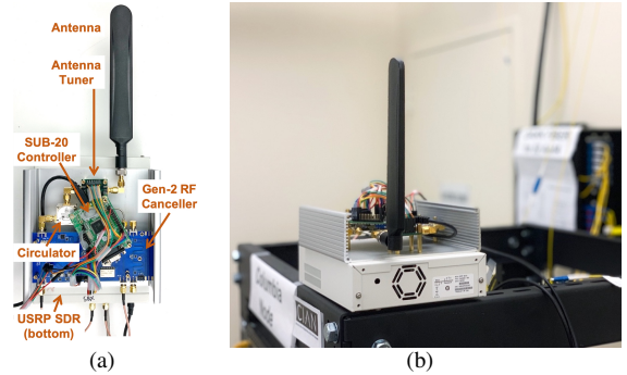
Fig. 2: (a) The implemented FlexICoN Gen-2 wideband FD radio, and (b) its integration with a COSMOS sandbox located at Columbia University, where the FD radio can be accessed and controlled by a COSMOS compute node (e.g., a host PC/server).
