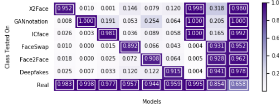
Fig. 6: Accuracies for Xception against all classes. Each column is a model with the trained classes outlined.
