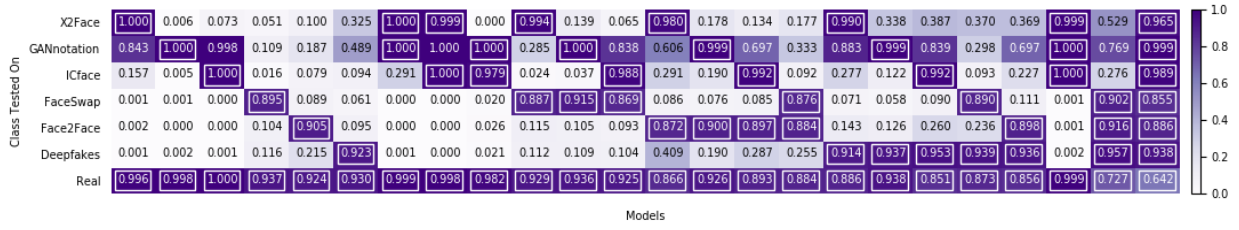
Fig. 5: Accuracies for Xception against all classes. Each column is a model with the trained classes outlined.
