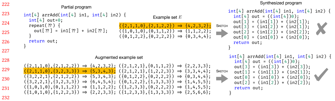
Fig. 3. Synthesizing a function to compute the sum of two arrays using SKETCH and SKETCHAX.
