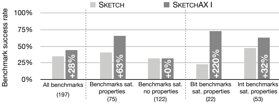
Fig. 6. Benchmark success rate of SKETCH and SKETCHAX I.
