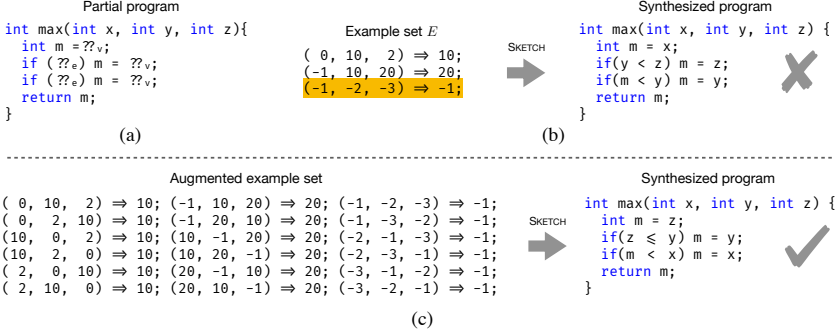
Fig. 1. Computing the maximum of three integers using SKETCH and SKETCHAX. The construct ??v is shorthand for the regular expression generator \{ |x|y|z|??| \} that defines a space of expressions equaling x or y or z or any integer constant. The construct ??e is shorthand for the regular expression generator (|max|x|y|z|) (< | \leq) (max|x|y|z) that defines a space of Boolean expressions with either a < or \leq operator, and operands equaling max or x or y or z .
