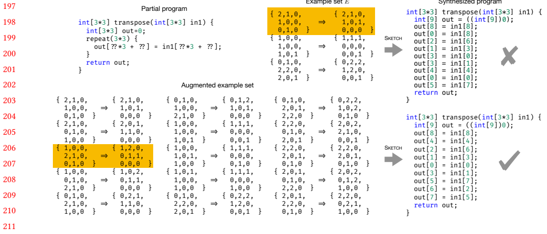
Fig. 2. Synthesizing a function to compute the transpose of a matrix using SKETCH and SKETCHAX.
