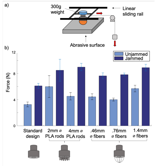
Fig. 2. Shear force tests. a) Shear setup. b) Passively and actively jammed shear strength before slipping on a pebbled surface.
