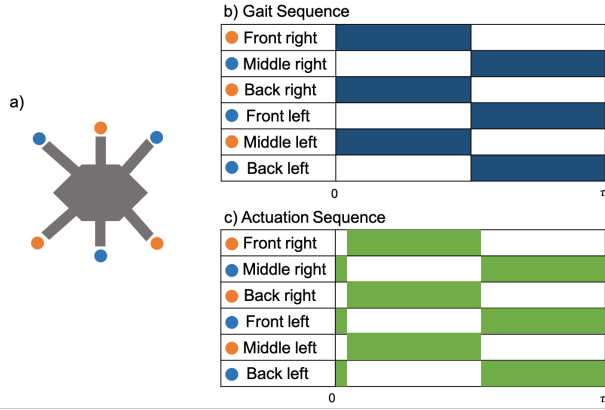
Fig. 5. Gait Sequence. a) Hexapod top view. Motion is from left to right. b,c) Actuation and gait sequences for one cycle of the hexapod gait. The shaded region corresponds to when the foot is in contact with the ground. The shaded region in the actuation sequence corresponds to when negative pressure is drawn. The non-shaded region in the actuation sequence corresponds to positive pressure.
